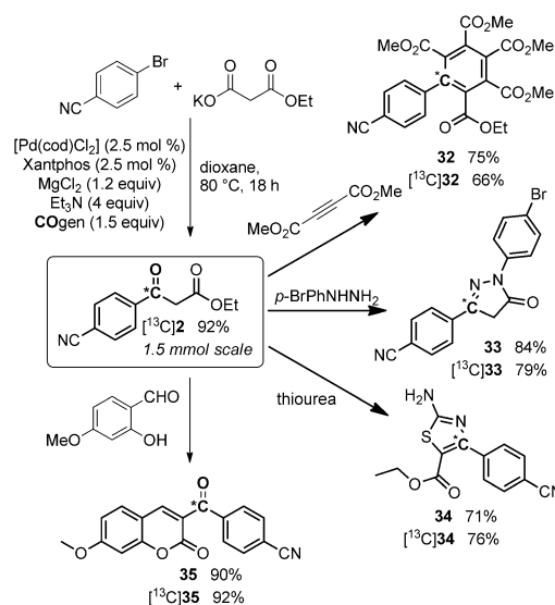
Scheme 7. Synthesis of ^{13}\text{C} -labeled \beta -keto ester 2 and the application of 2 and [\text{C}^{13}]\text{2} in cyclization reactions.
