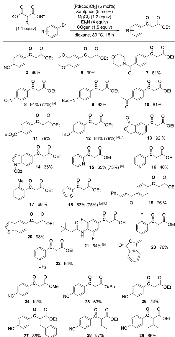
Scheme 3. Carbonylative arylation of monoethyl potassium malonate with aryl halides. Reaction conditions: Chamber A: Aryl bromide (0.3 mmol), [Pd(cod)Cl 2 ] (0.015 mmol), Xantphos (0.015 mmol), monoethyl potassium malonate (0.33 mmol), MgCl 2 (0.36 mmol), Et 3 N (1.2 mmol), and dioxane (3 mL) at 80 °C. Chamber B: COgen (0.45 mmol), Cy 2 NMe (0.9 mmol), [Pd(cod)Cl 2 ] (0.023 mmol), P( t Bu) 3 HBF 4 (0.023 mmol), and dioxane (3 mL) at 80 °C for 18 h. [a] Yields in parentheses were obtained from reactions run with Pd(OAc) 2 . [b] Reaction run at 100 °C in butyronitrile with Cy 2 NMe as the base.
